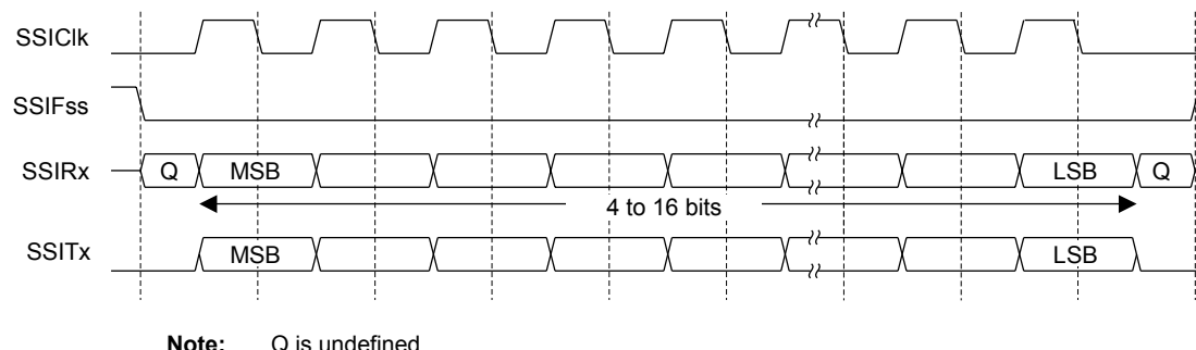
Figure 13-6. Freescale SPI Frame Format with SPO=0 and SPH=1
